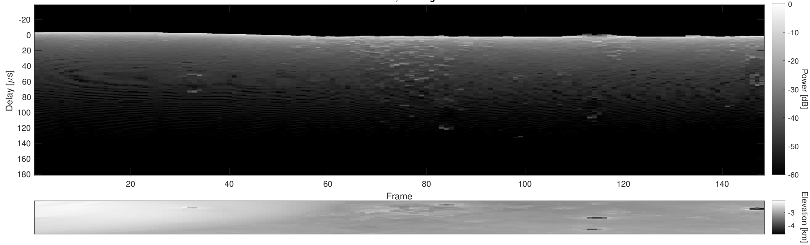
Orbit 18352, Cluttergram
