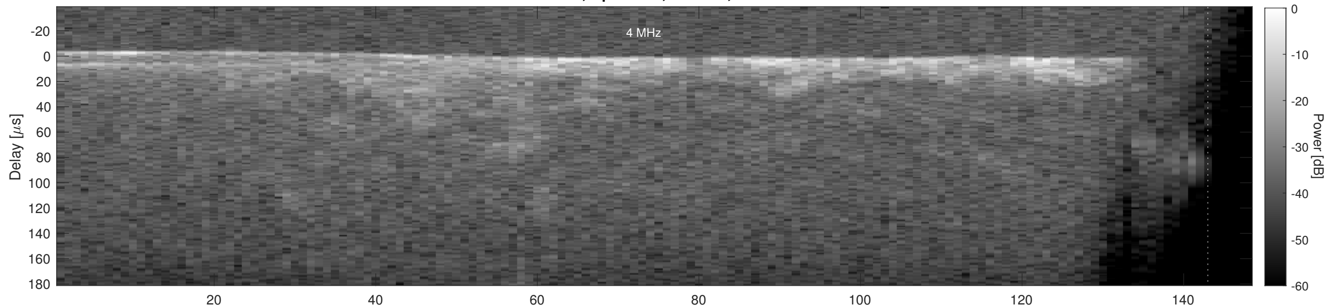
Orbit 18352, Cluttergram
