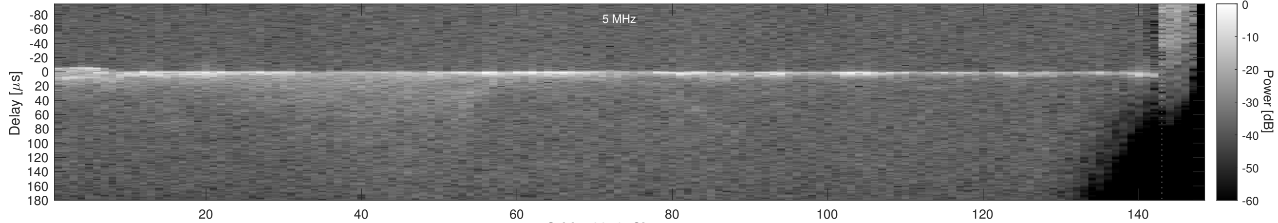
Orbit 18356, Cluttergram
