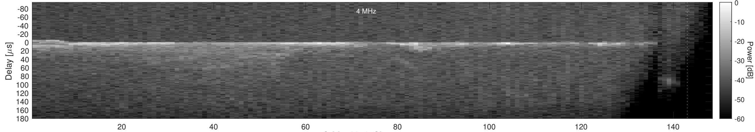
Orbit 18356, Cluttergram
