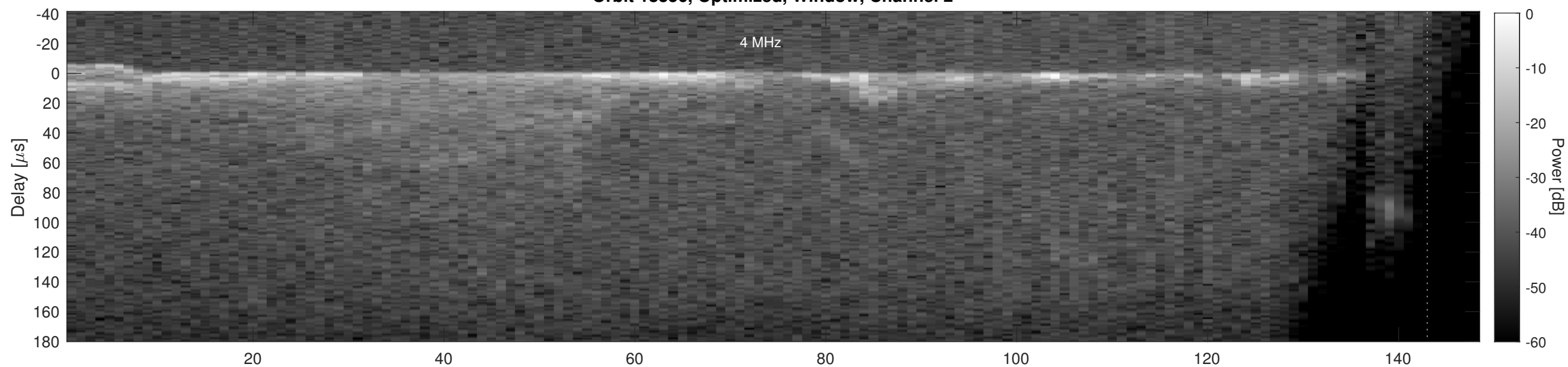
Orbit 18356, Cluttergram
