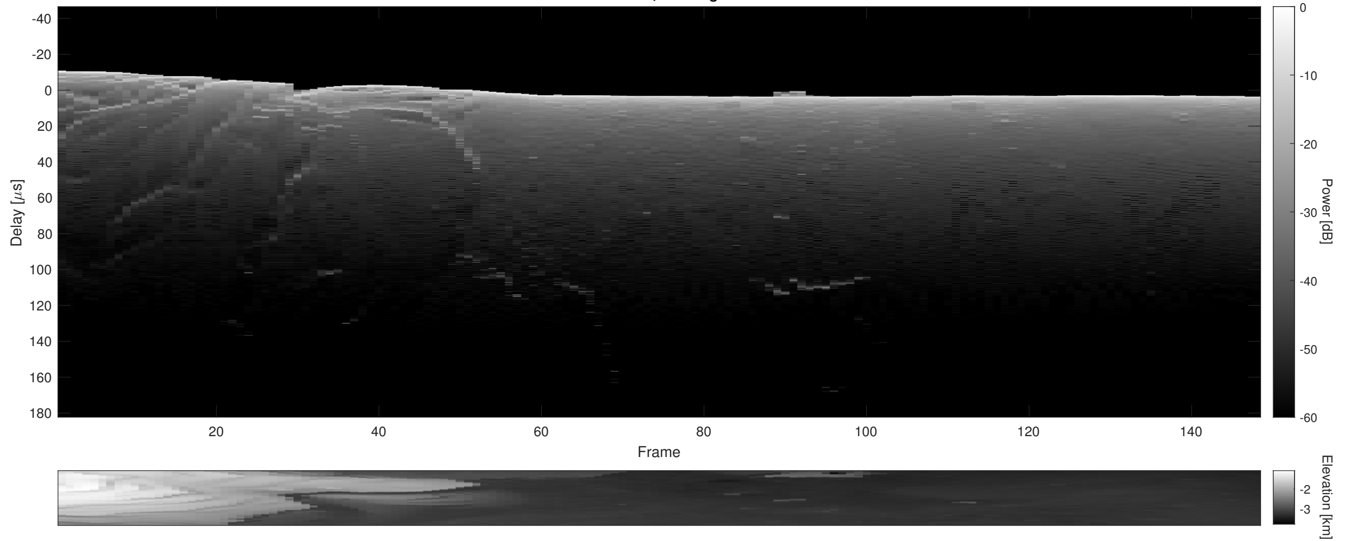
Orbit 18358, Cluttergram
