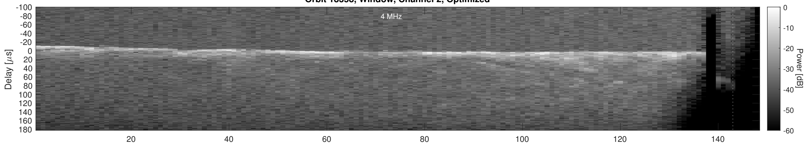
Orbit 18358, Cluttergram
