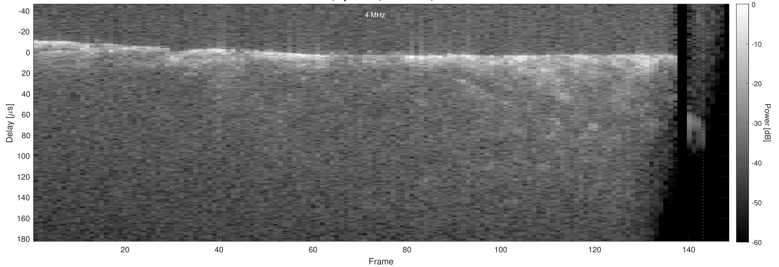
Orbit 18358, Optimized, No Window, Channel 2
