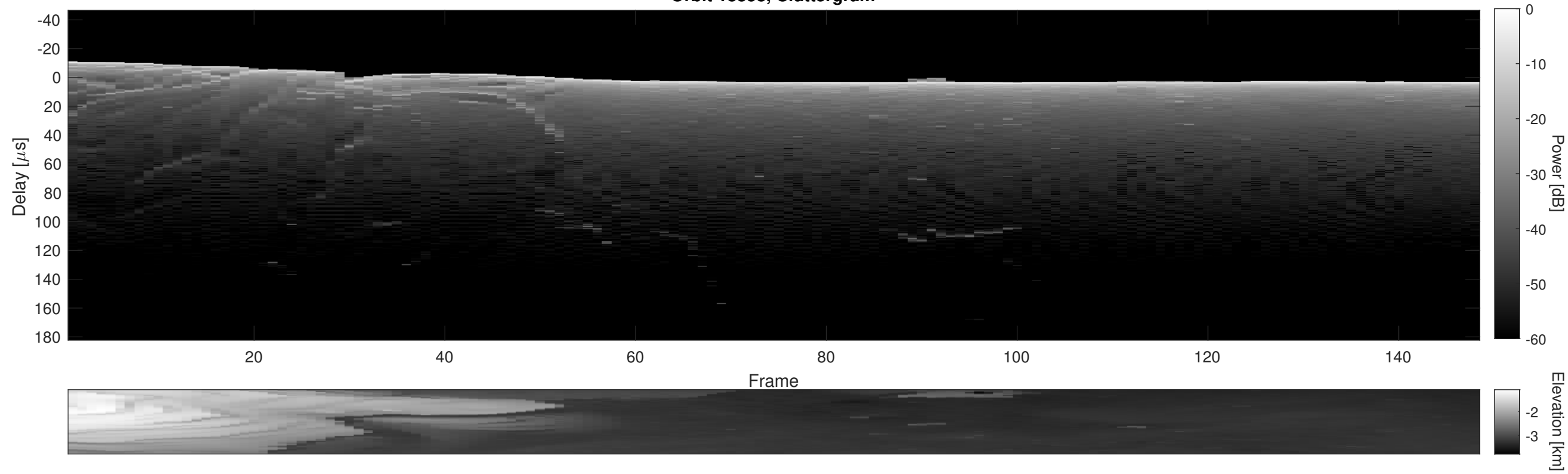
Orbit 18358, Cluttergram
