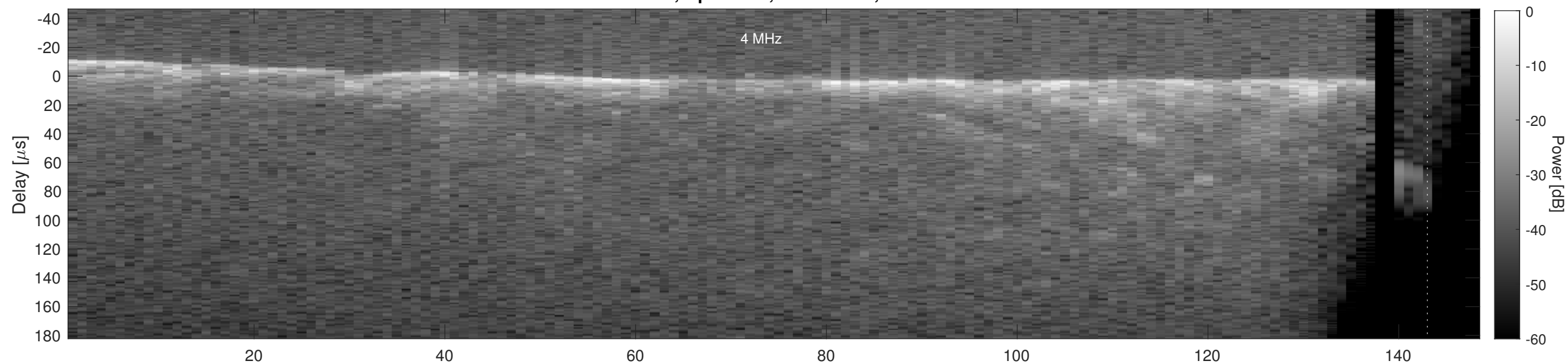
Orbit 18358, Cluttergram
