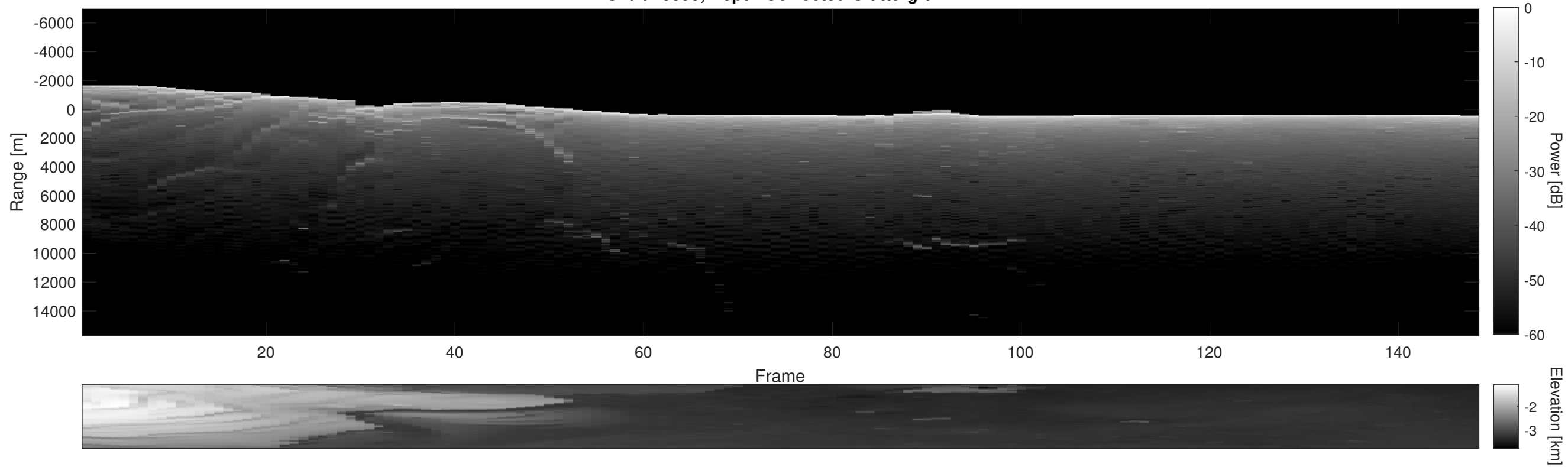
Orbit 18358, Depth-Corrected Cluttergram
