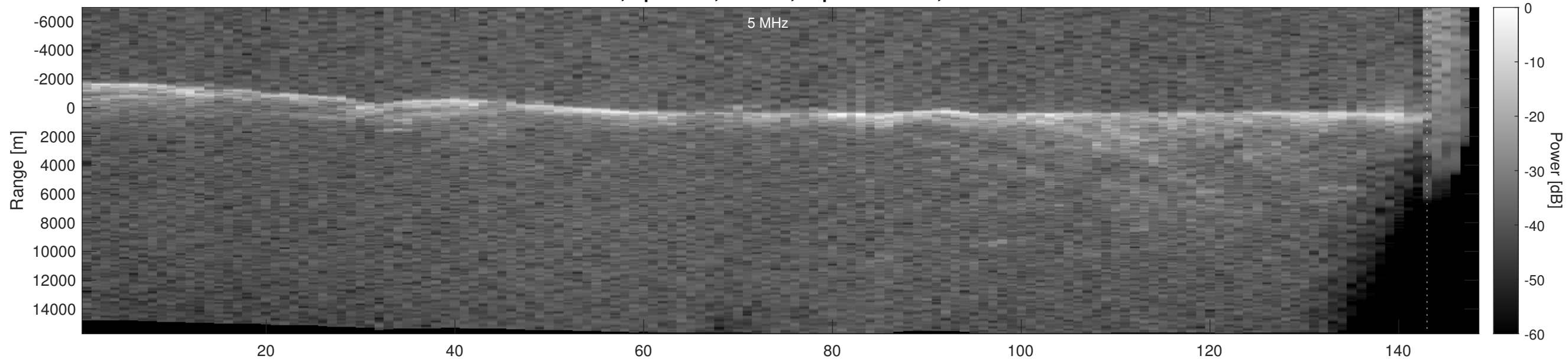
Orbit 18358, Optimized, Window, Depth-Corrected, Channel 2
