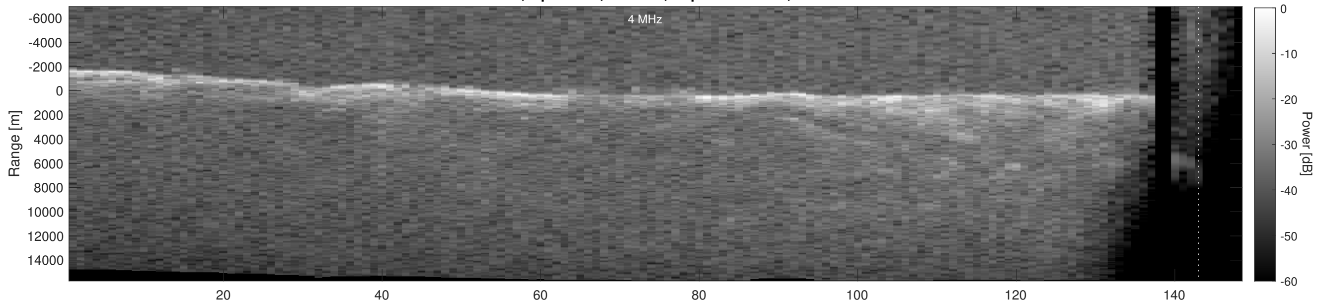
Orbit 18358, Depth-Corrected Cluttergram
