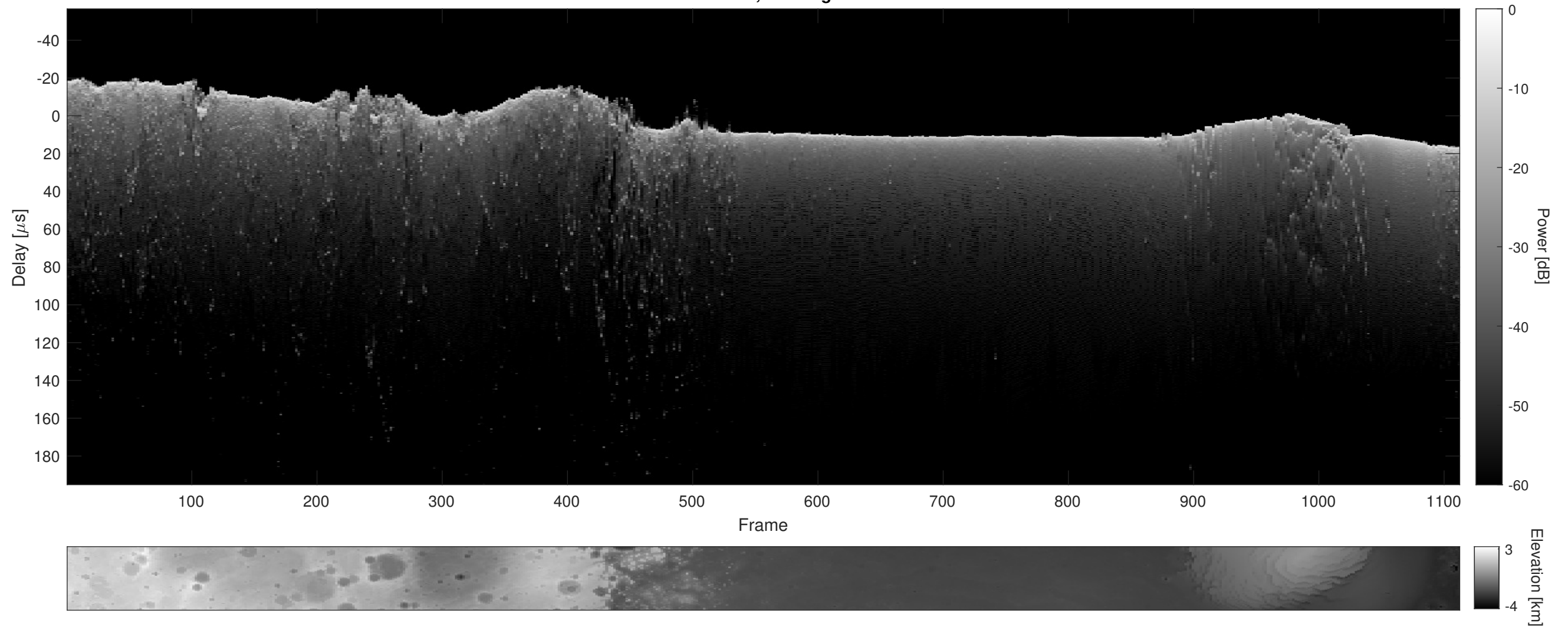
Orbit 18387, Cluttergram
