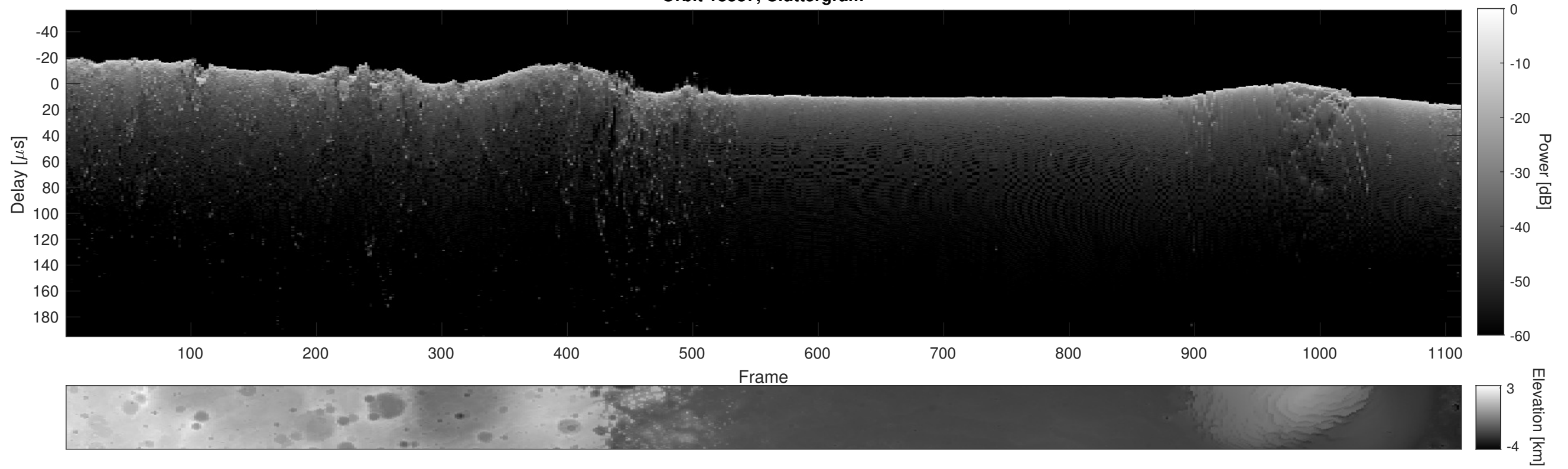
Orbit 18387, Cluttergram
