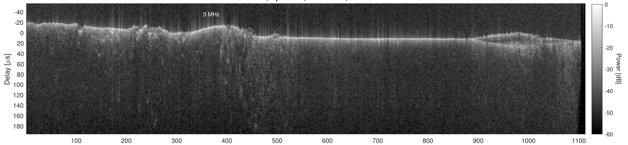
Orbit 18387, Cluttergram
