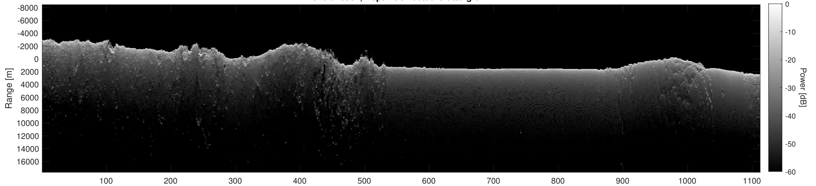
Orbit 18387, Depth-Corrected Cluttergram
