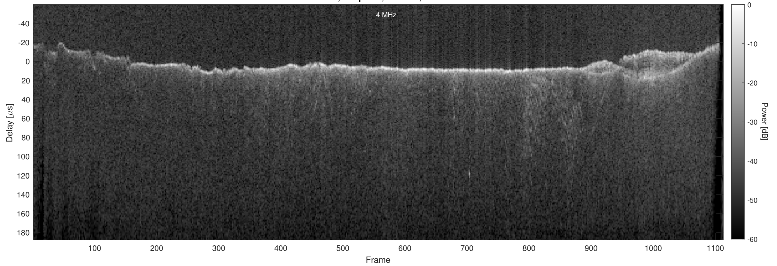
Orbit 18388, Chapman, Window, Channel 2
