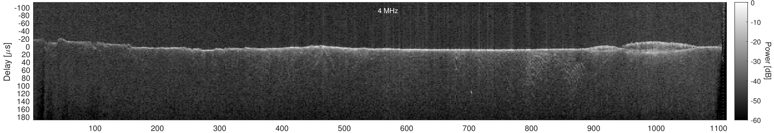
Orbit 18388, Cluttergram
