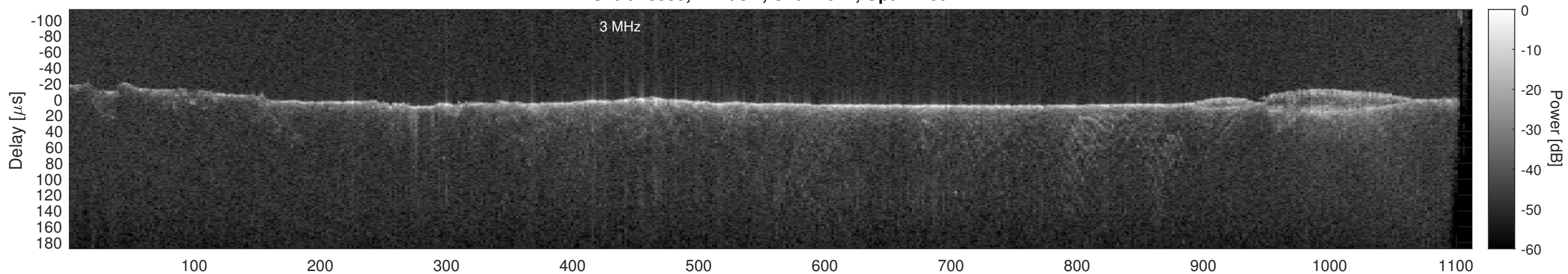
Orbit 18388, Cluttergram
