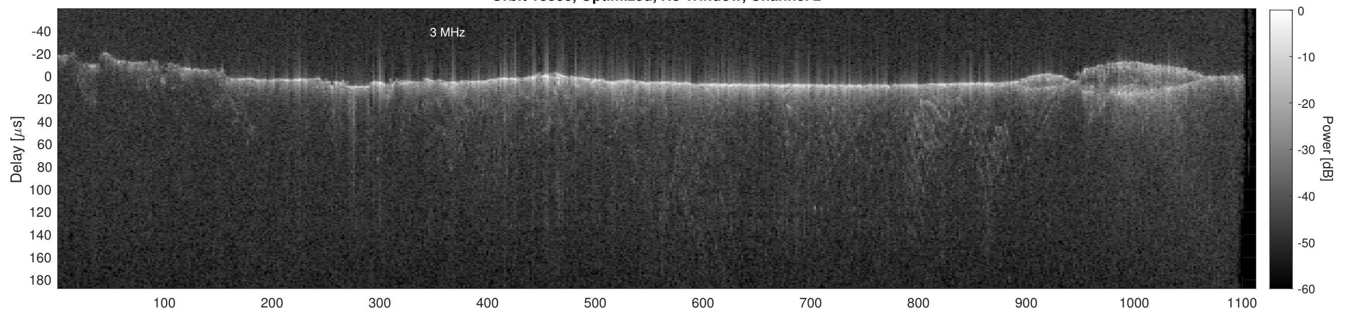
Orbit 18388, Cluttergram
