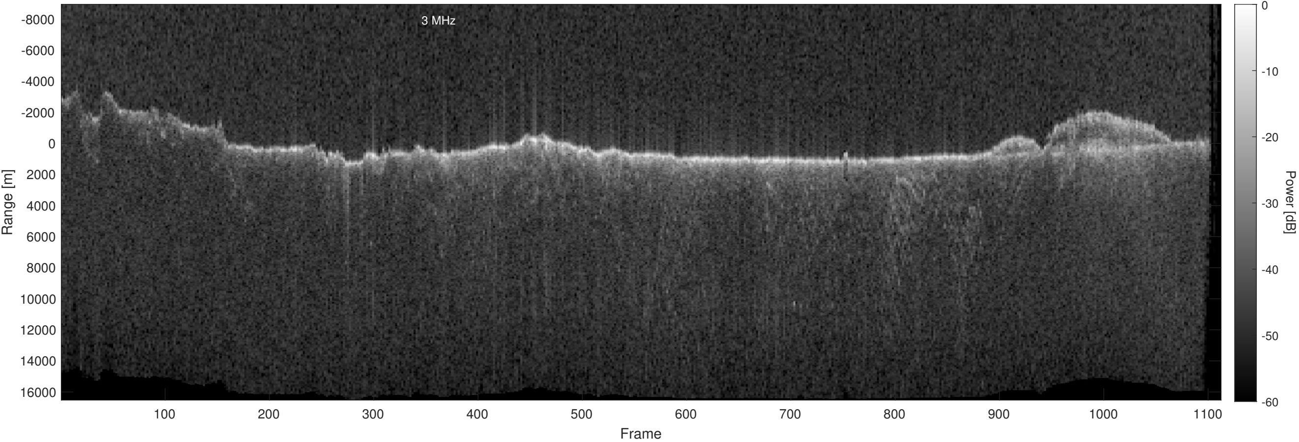
Orbit 18388, Optimized, Window, Depth-Corrected, Channel 2
