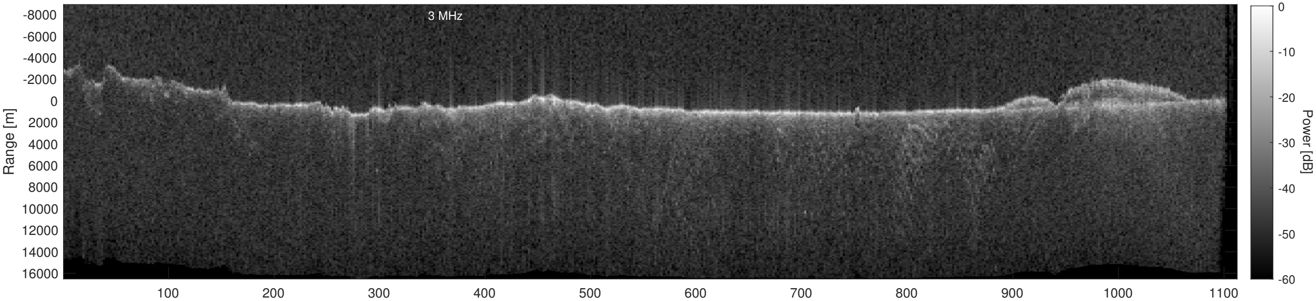
Orbit 18388, Depth-Corrected Cluttergram
