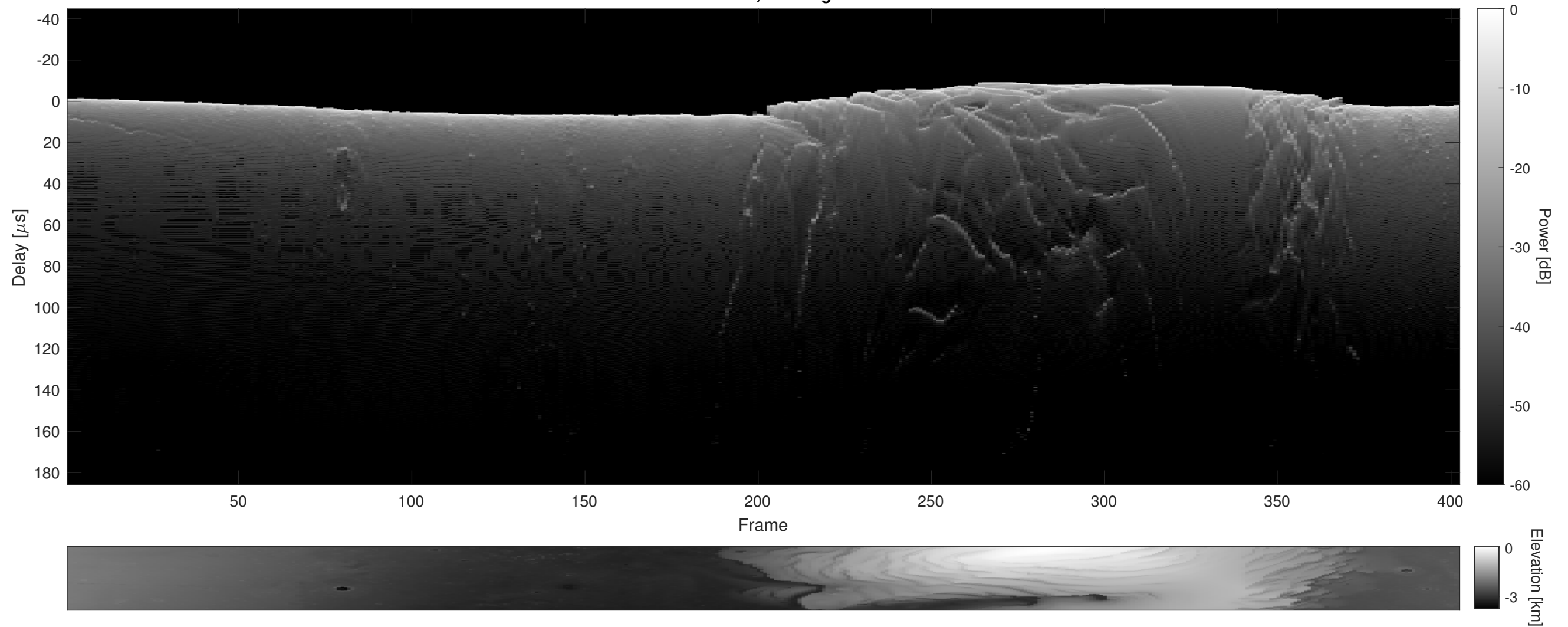
Orbit 18392, Cluttergram
