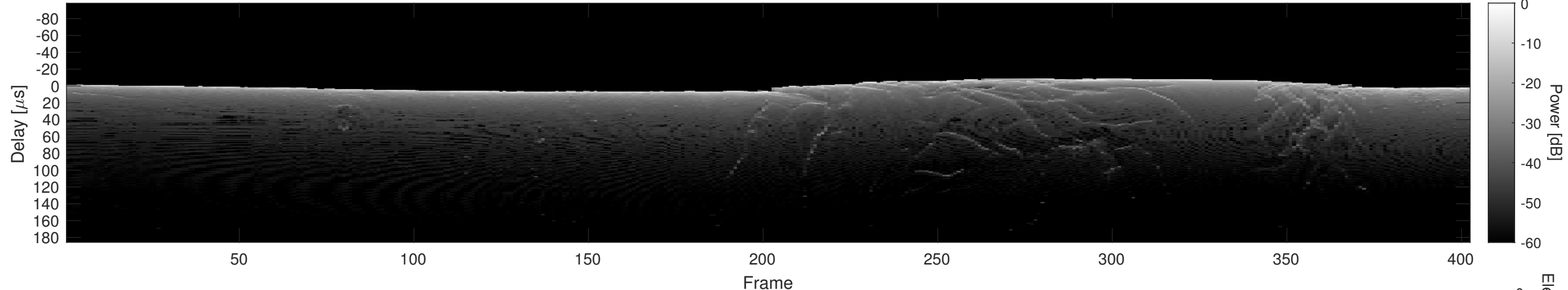
Orbit 18392, Cluttergram
