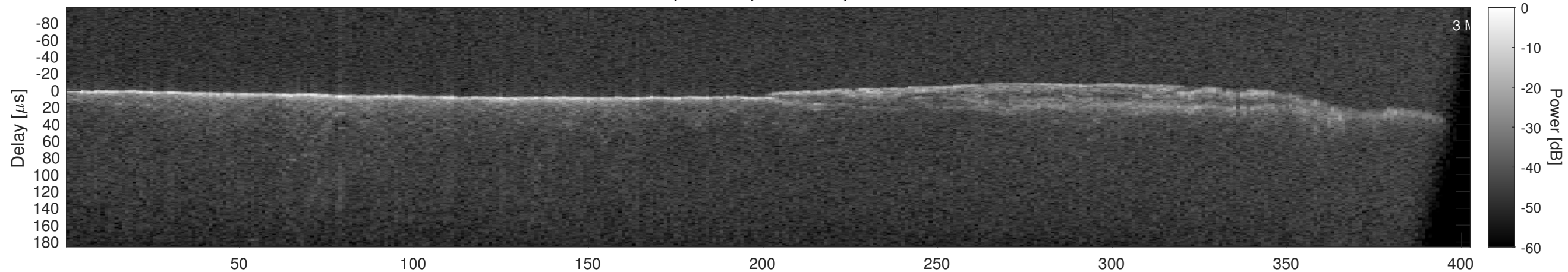
Orbit 18392, Window, Channel 2, Chapman
