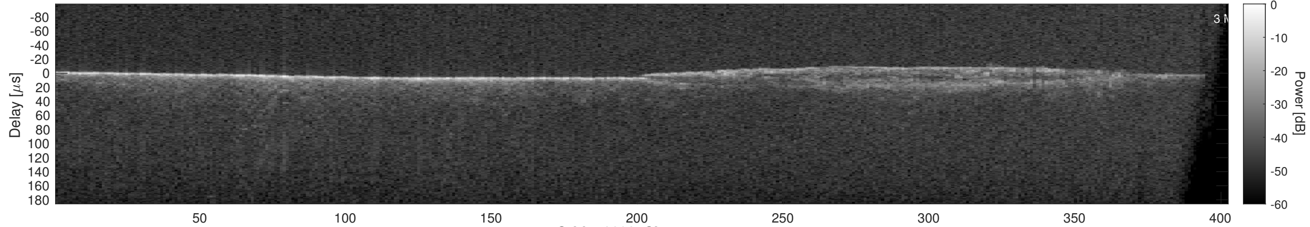
Orbit 18392, Cluttergram
