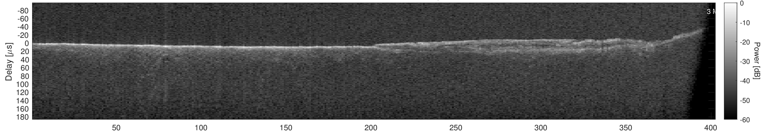
Orbit 18392, Window, Channel 2, Optimized
