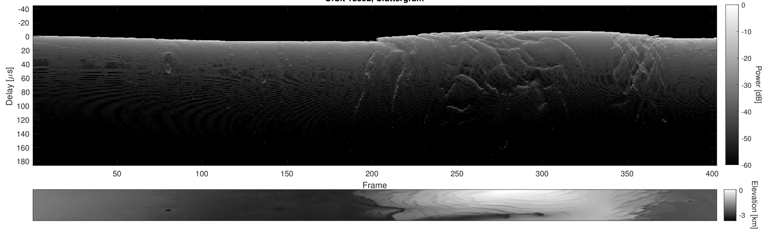
Orbit 18392, Cluttergram
