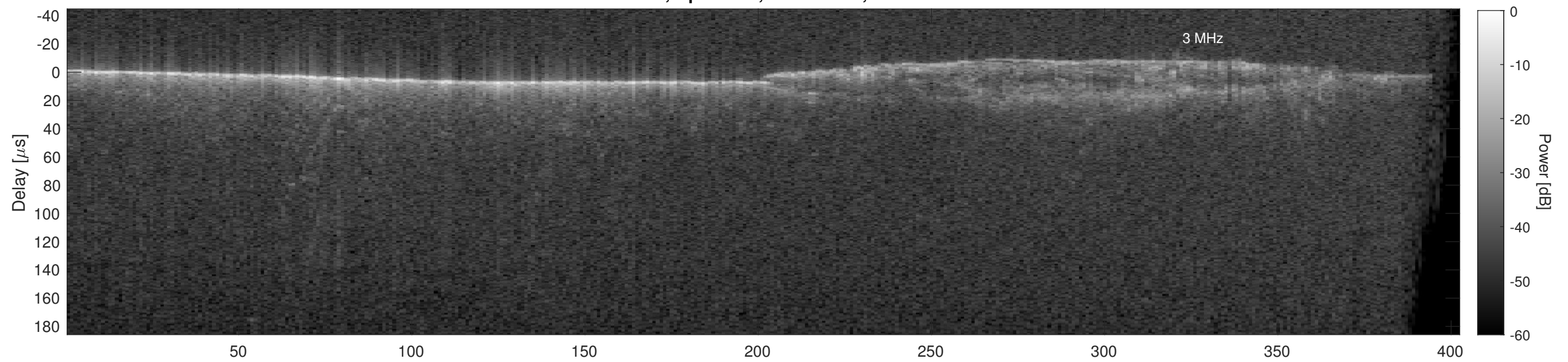
Orbit 18392, Cluttergram
