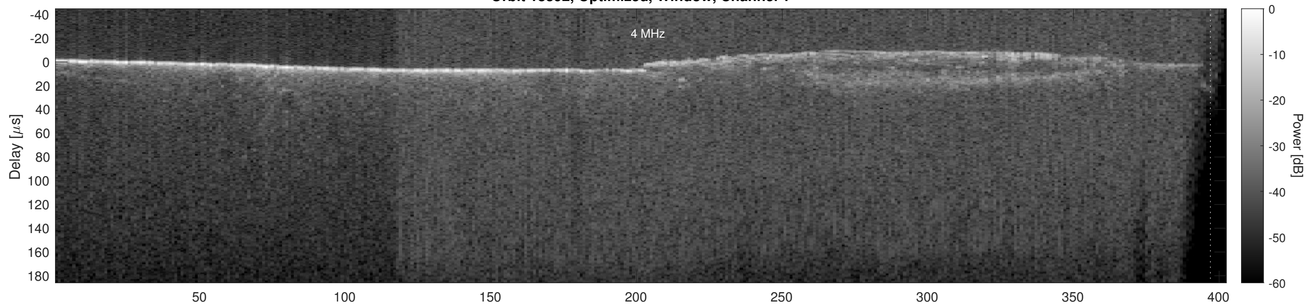
Orbit 18392, Optimized, Window, Channel 2
