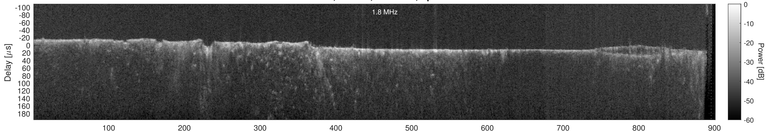
Orbit 18394, Cluttergram
