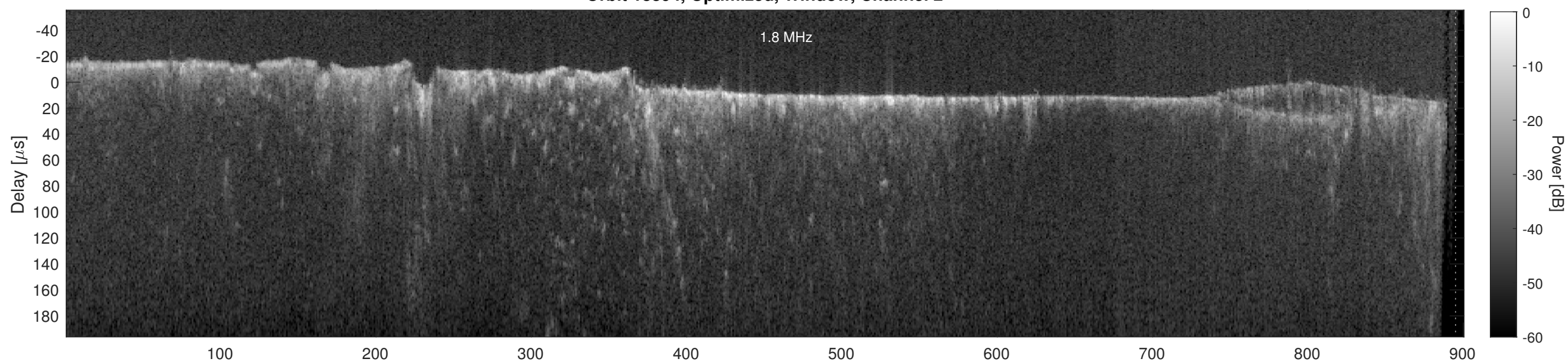
Orbit 18394, Cluttergram
