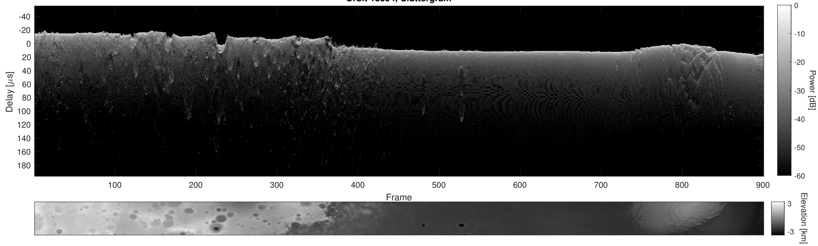
Orbit 18394, Cluttergram
