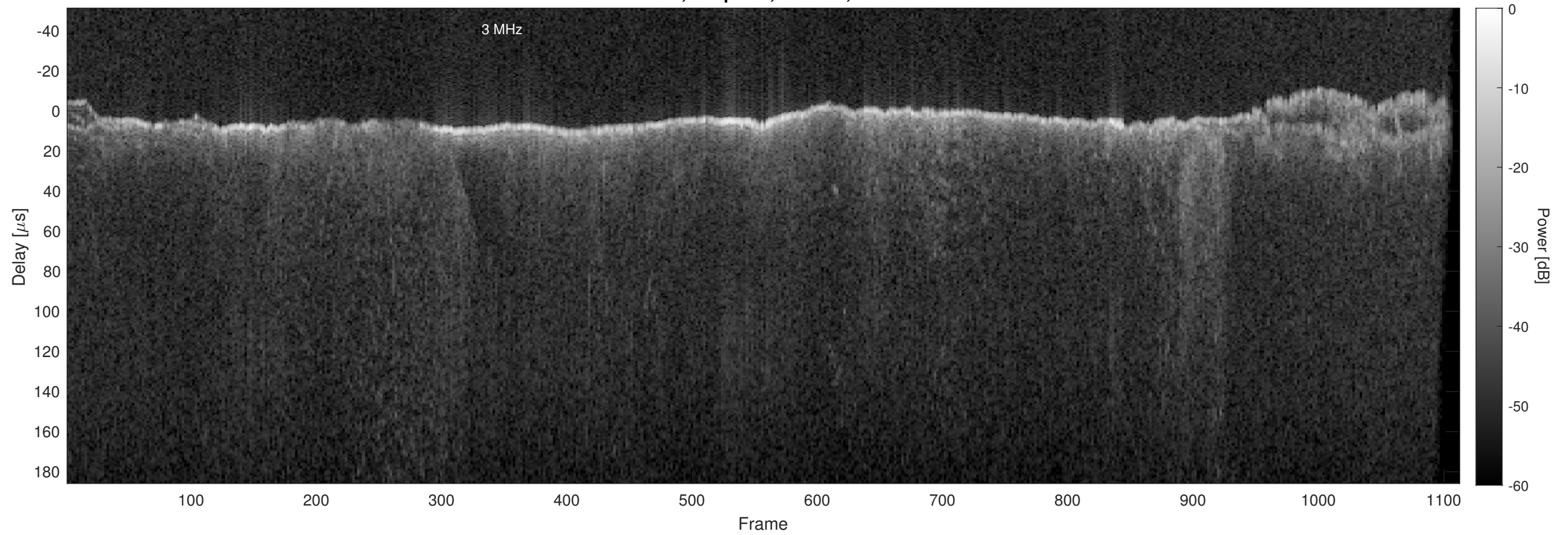
Orbit 18396, Chapman, Window, Channel 2
