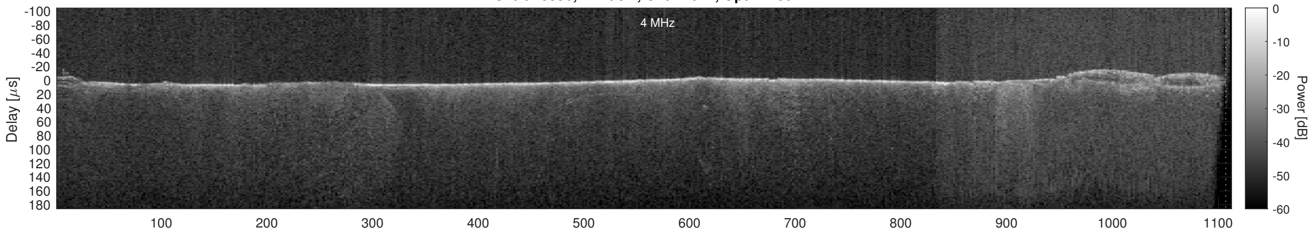
Orbit 18396, Cluttergram
