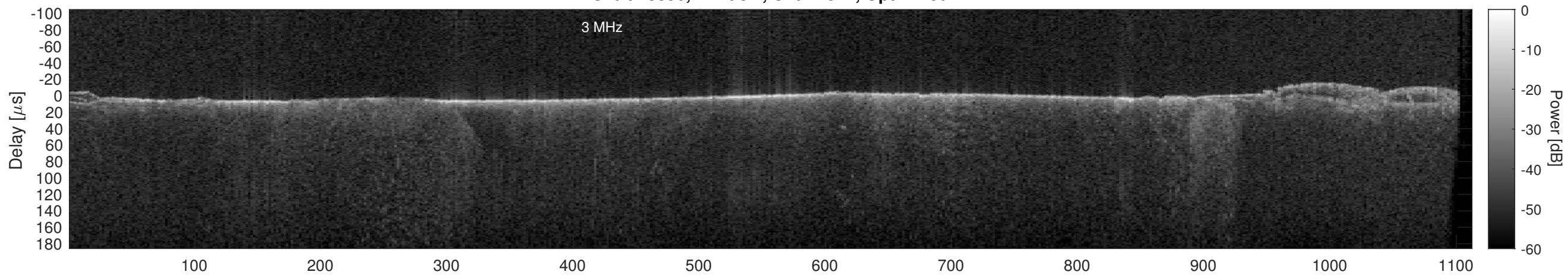
Orbit 18396, Cluttergram
