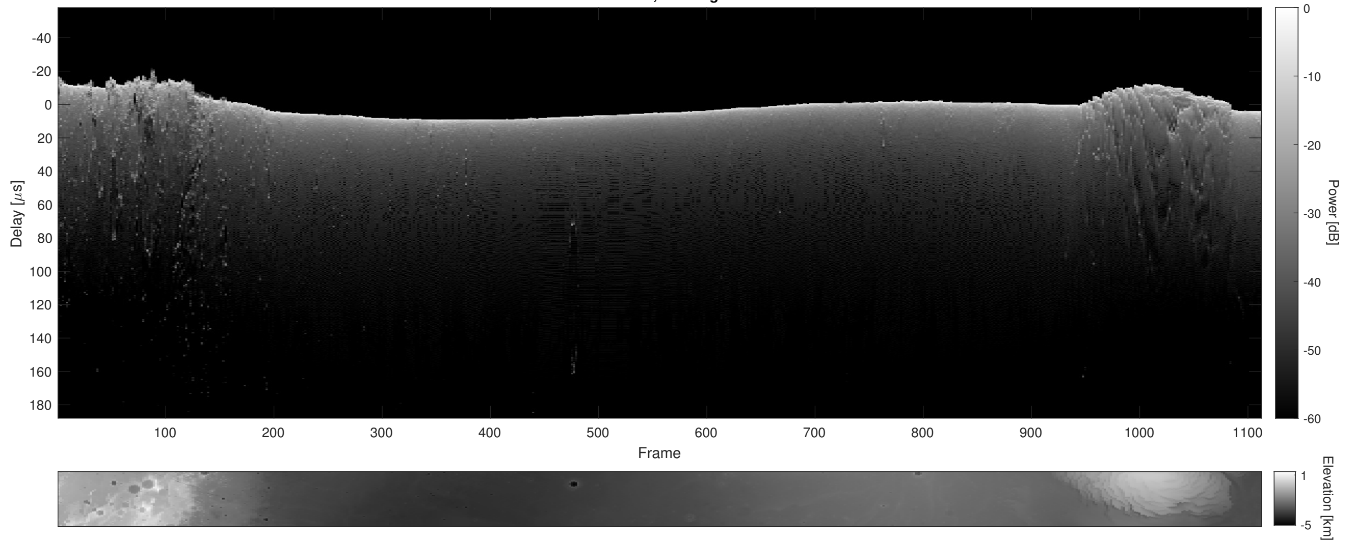
Orbit 18397, Cluttergram
