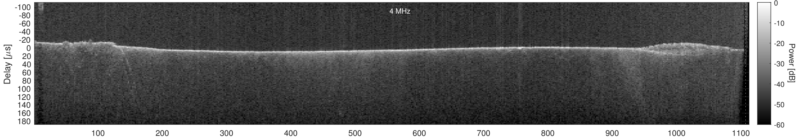
Orbit 18397, Cluttergram
