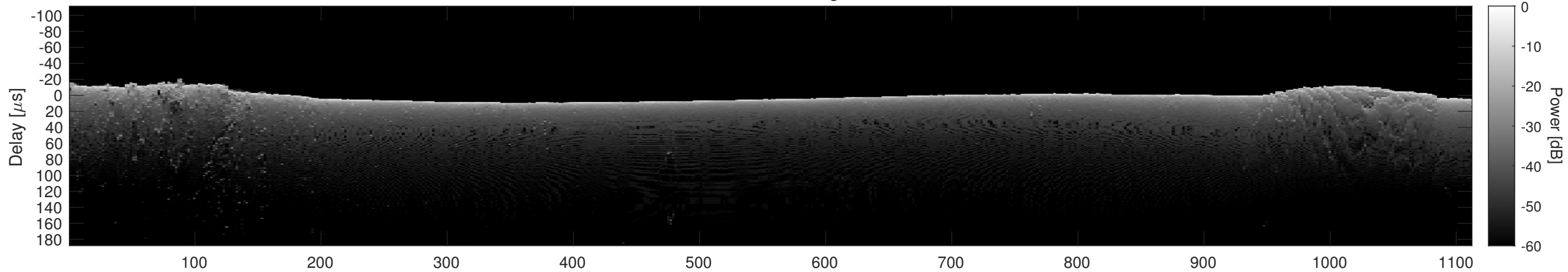
Orbit 18397, Cluttergram
