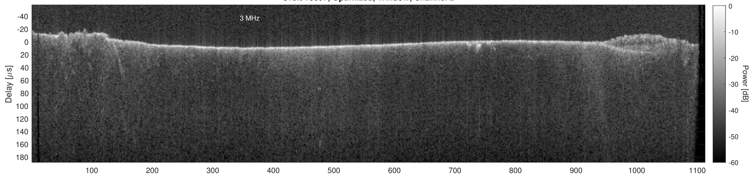
Orbit 18397, Cluttergram
