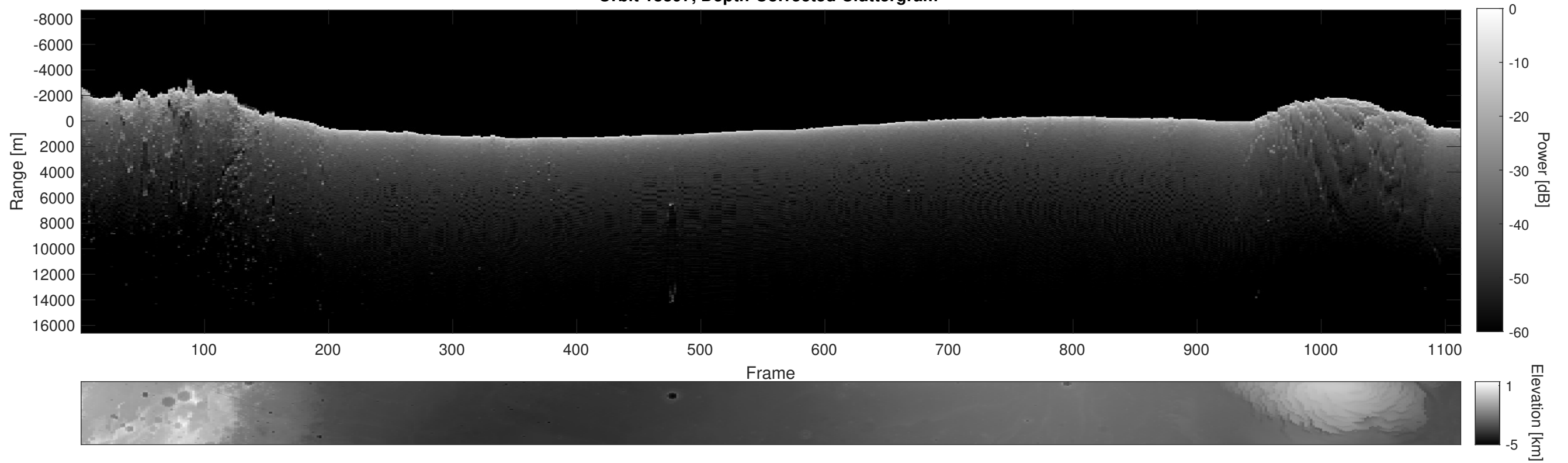
Orbit 18397, Depth-Corrected Cluttergram
