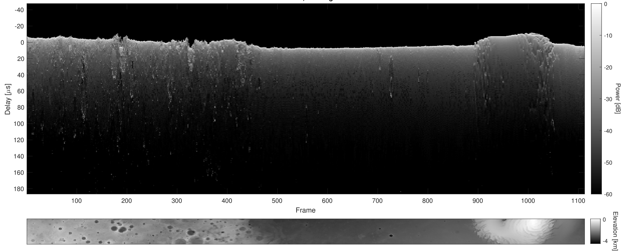
Orbit 18398, Cluttergram
