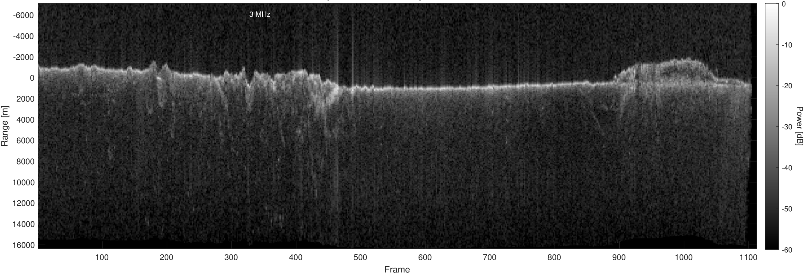
Orbit 18398, Optimized, Window, Depth-Corrected, Channel 2
