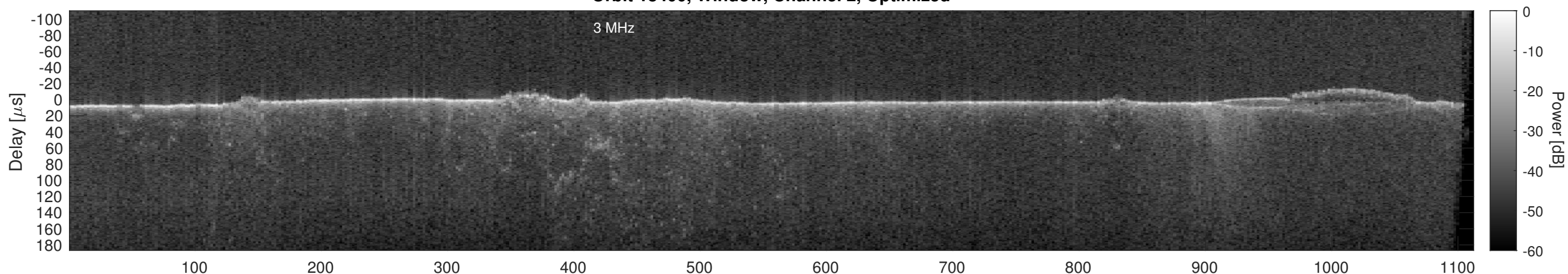
Orbit 18400, Cluttergram
