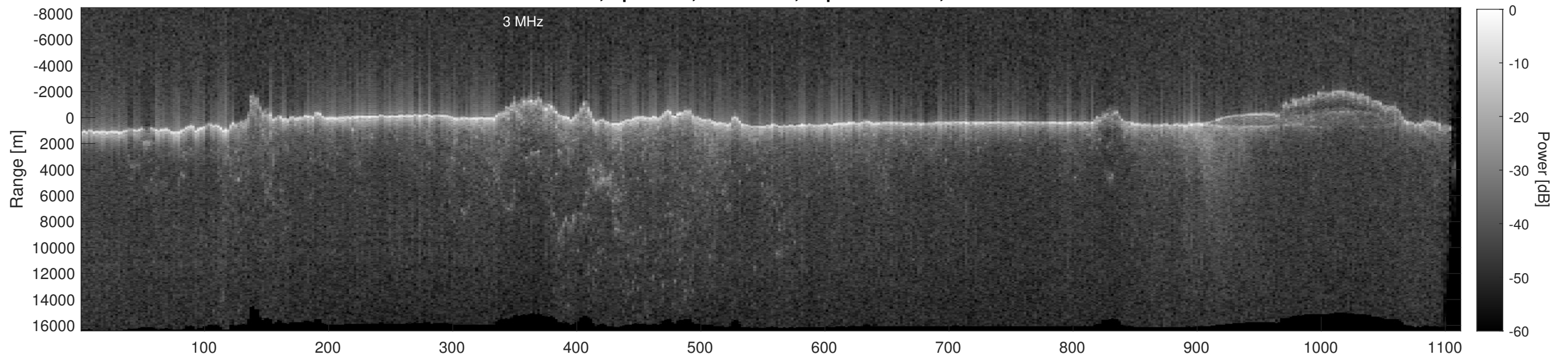
Orbit 18400, Depth-Corrected Cluttergram
