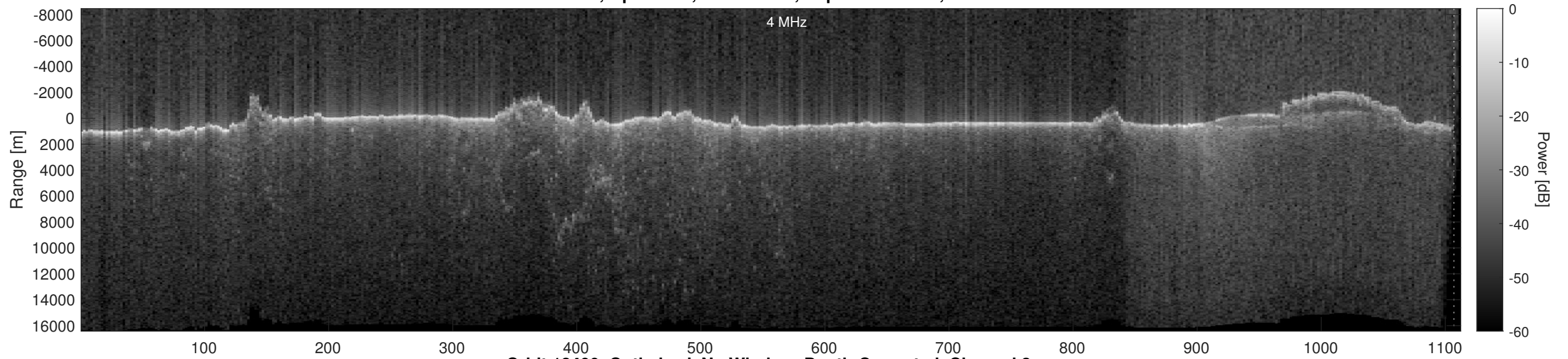
Orbit 18400, Optimized, No Window, Depth-Corrected, Channel 2
