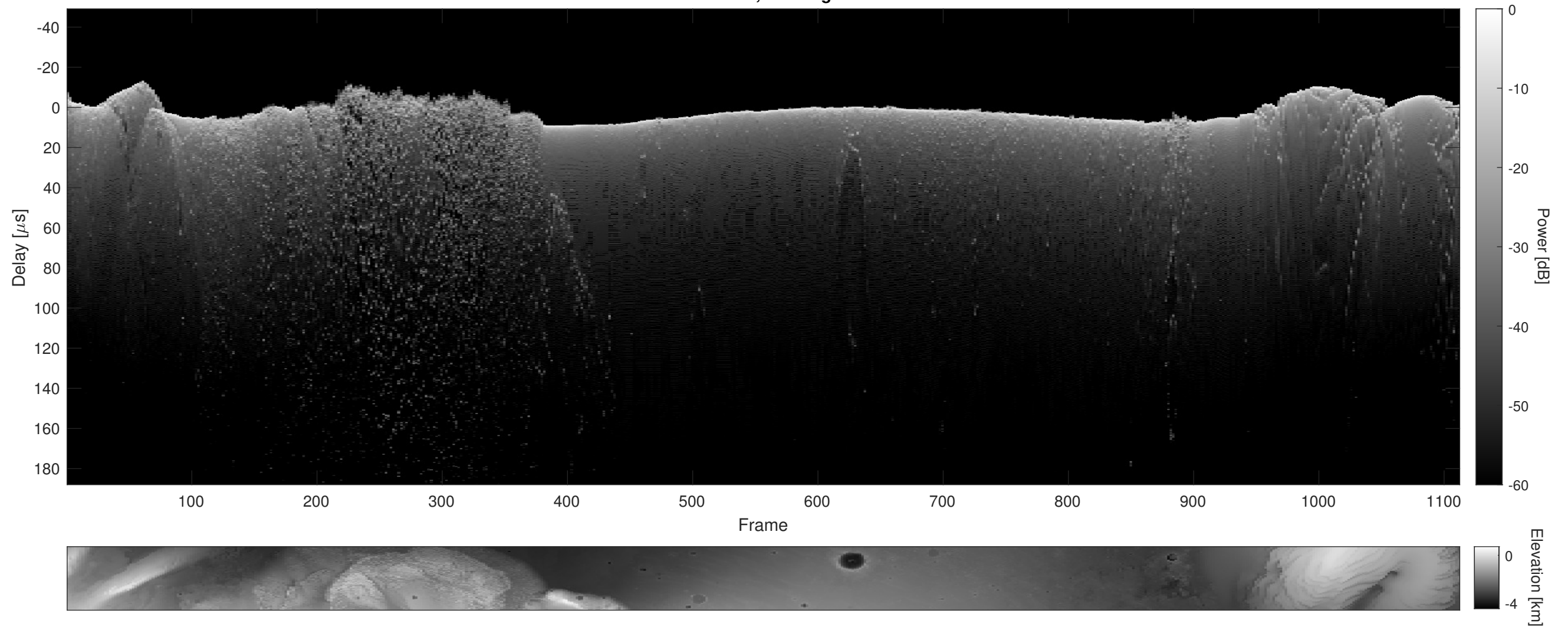
Orbit 18403, Cluttergram
