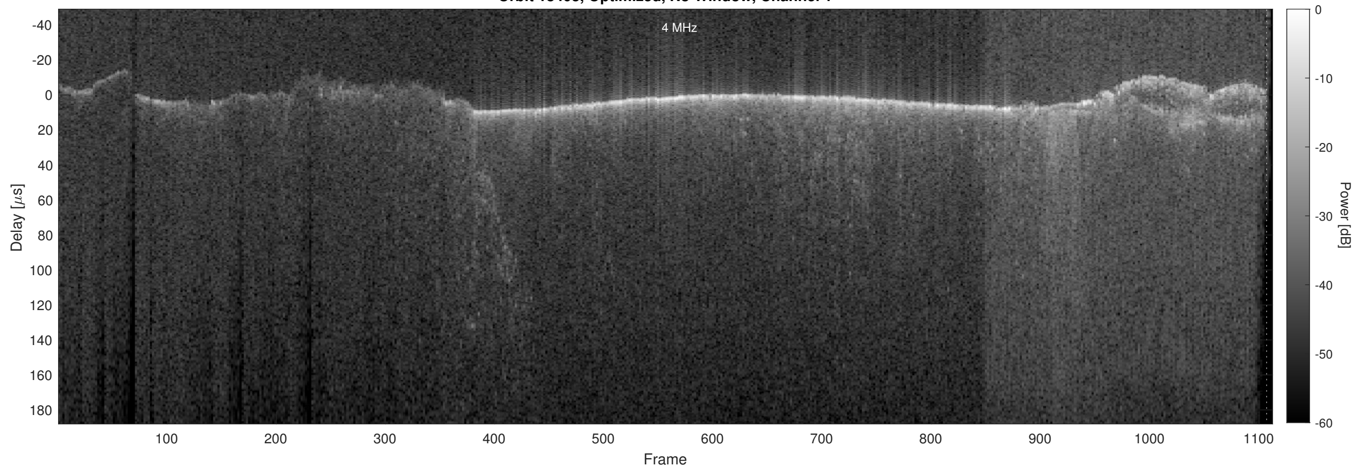
Orbit 18403, Optimized, No Window, Channel 2
