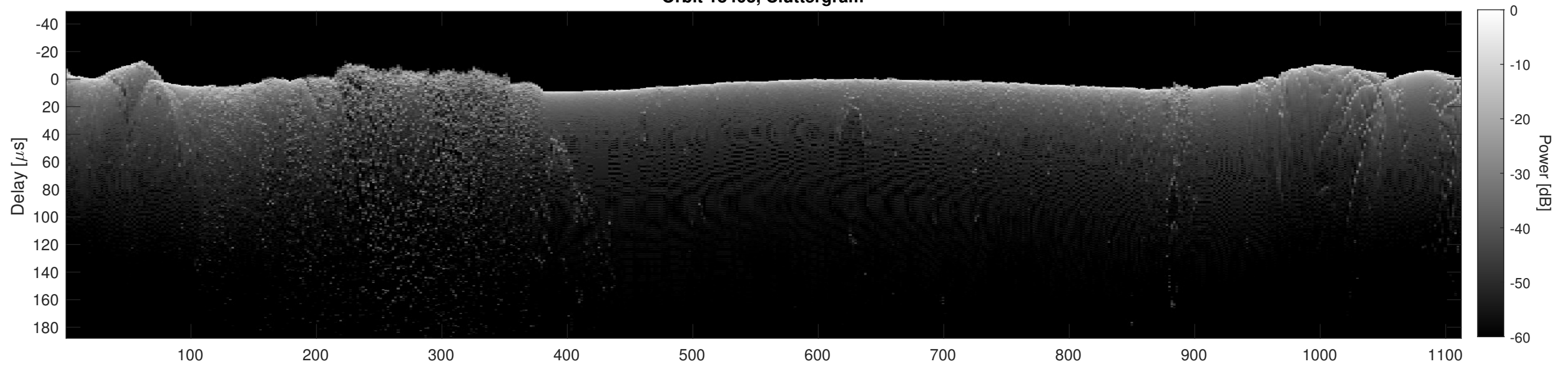
Orbit 18403, Cluttergram
