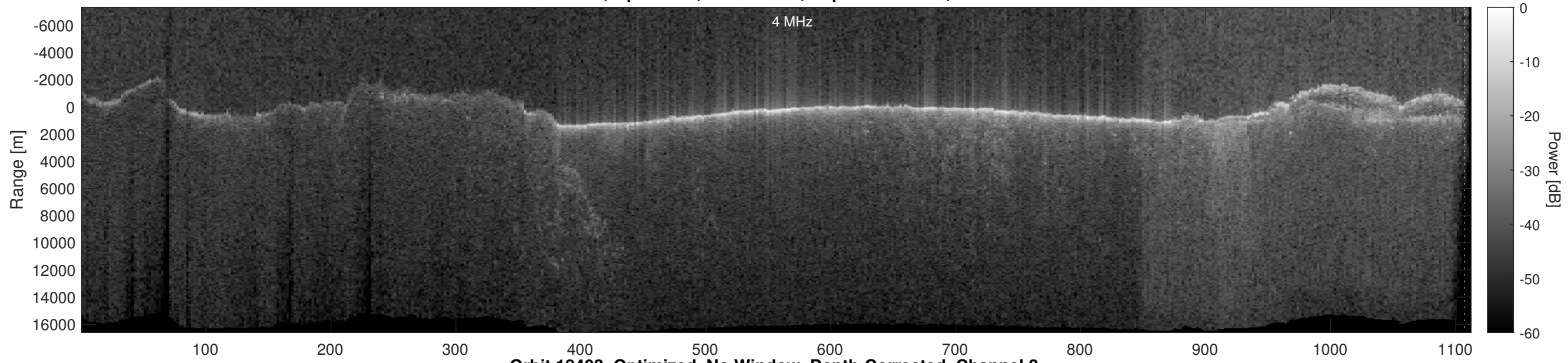
Orbit 18403, Optimized, No Window, Depth-Corrected, Channel 2
