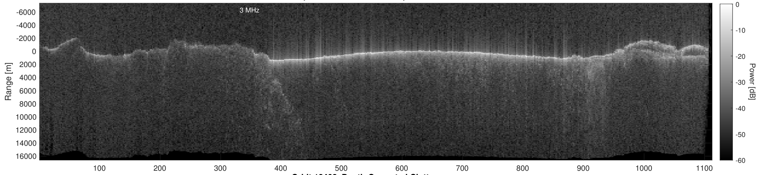
Orbit 18403, Depth-Corrected Cluttergram
