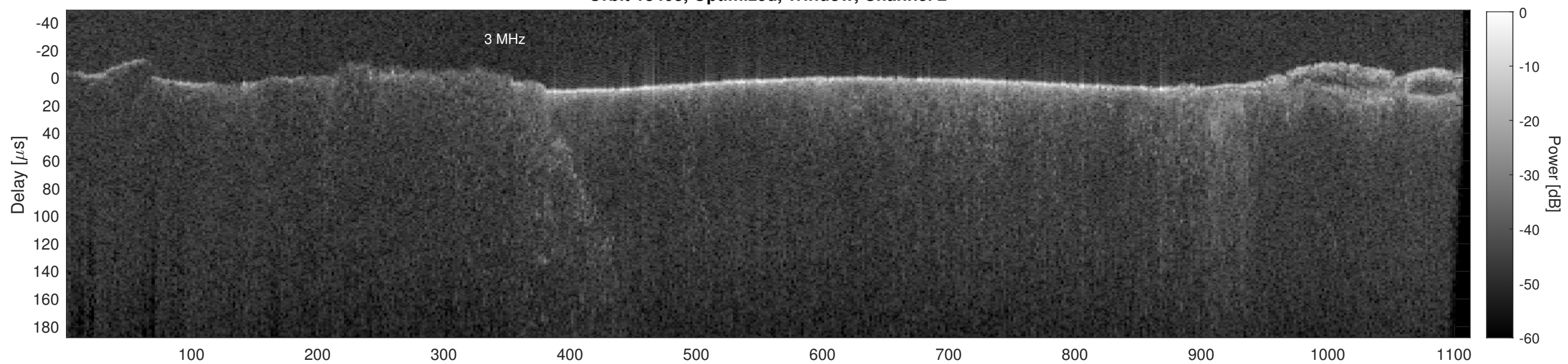
Orbit 18403, Cluttergram
