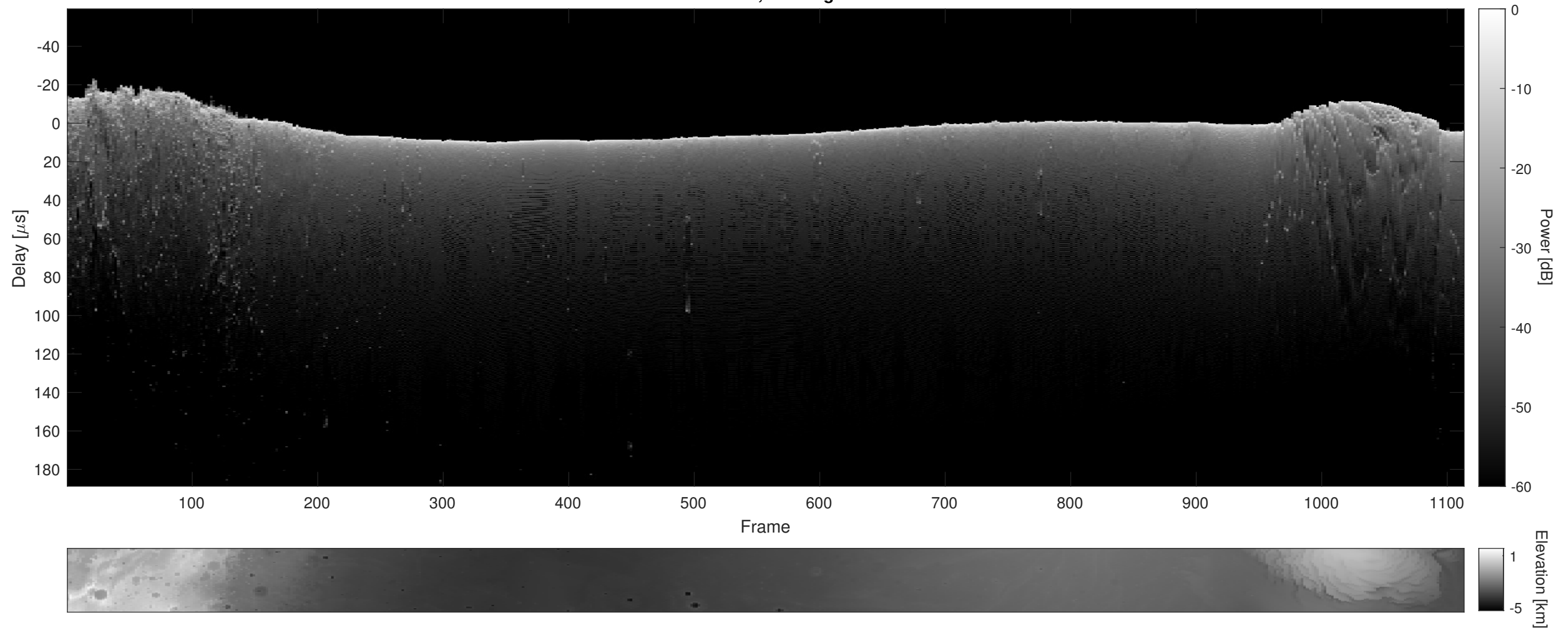
Orbit 18404, Cluttergram
