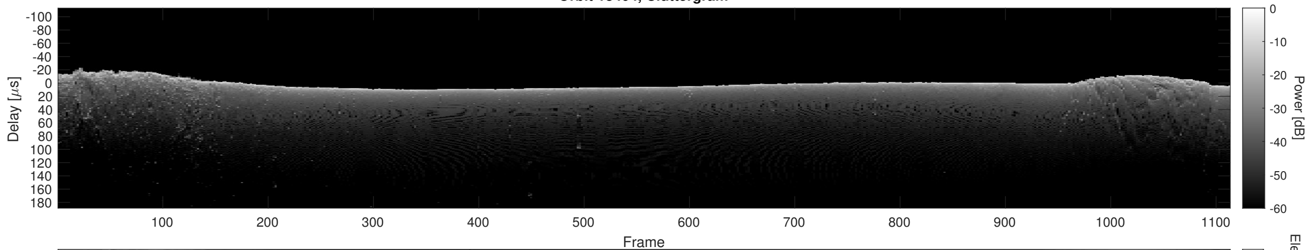
Orbit 18404, Cluttergram
