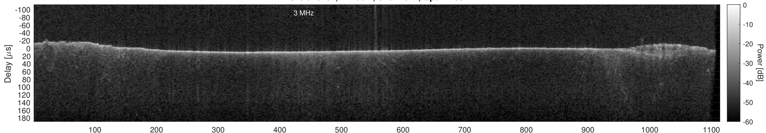
Orbit 18404, Cluttergram
