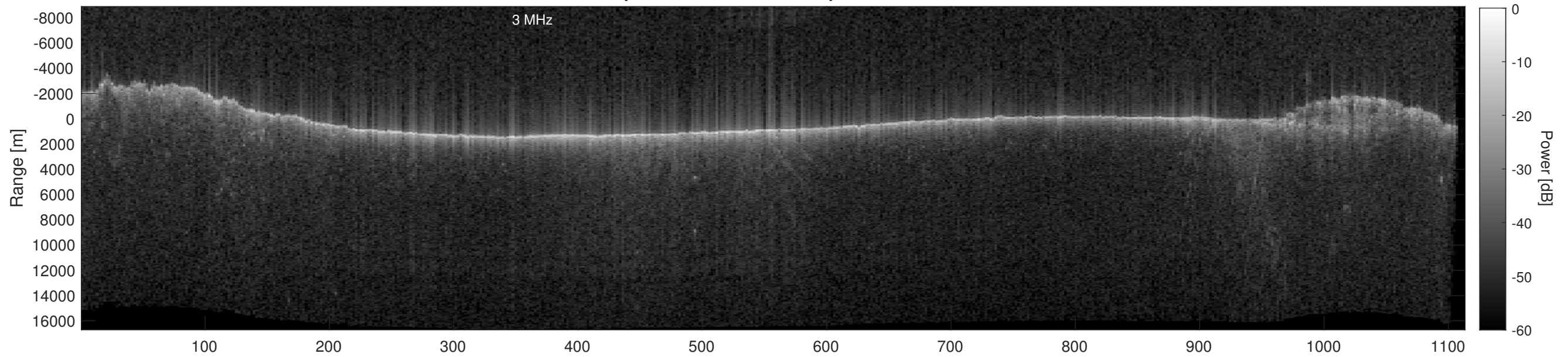
Orbit 18404, Depth-Corrected Cluttergram
