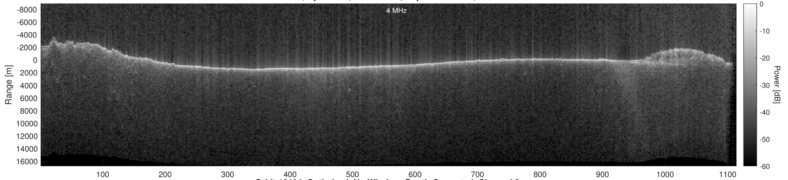
Orbit 18404, Optimized, No Window, Depth-Corrected, Channel 2
