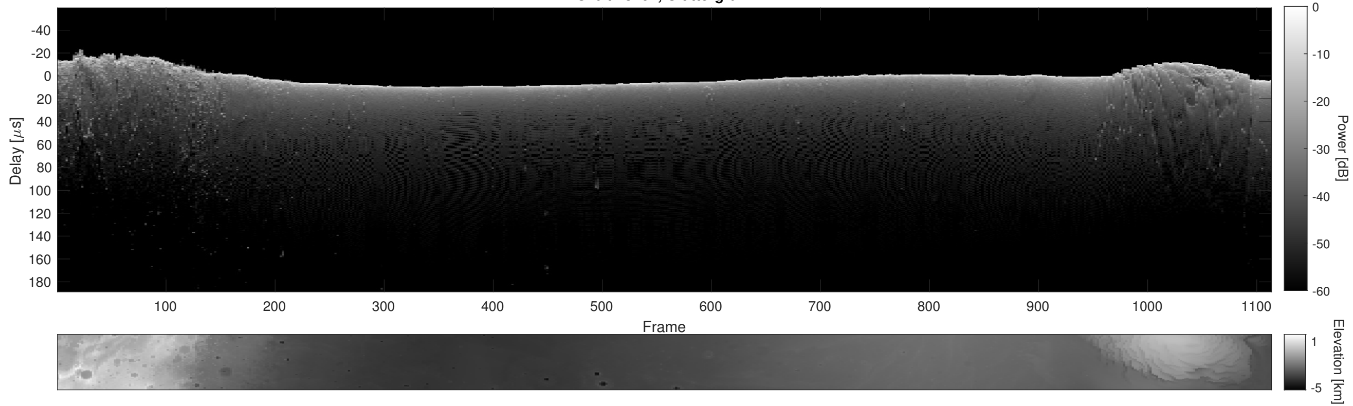
Orbit 18404, Cluttergram
