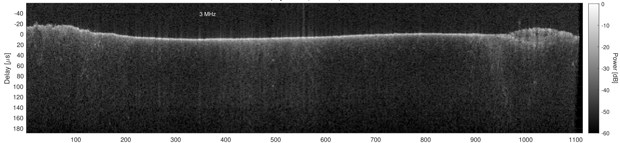
Orbit 18404, Cluttergram
