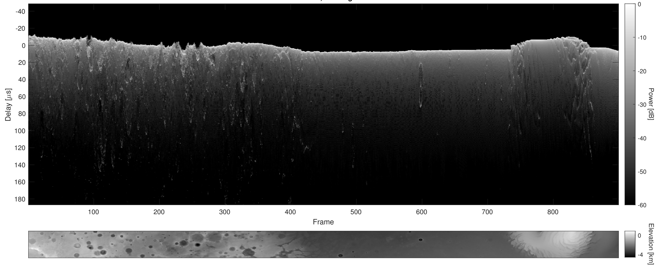
Orbit 18405, Cluttergram
