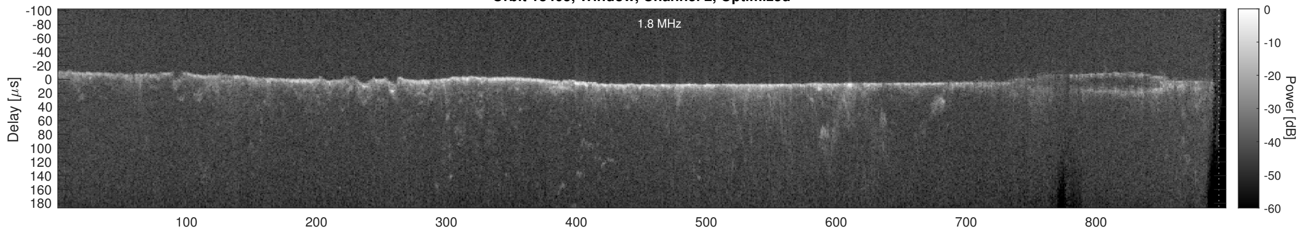
Orbit 18405, Cluttergram
