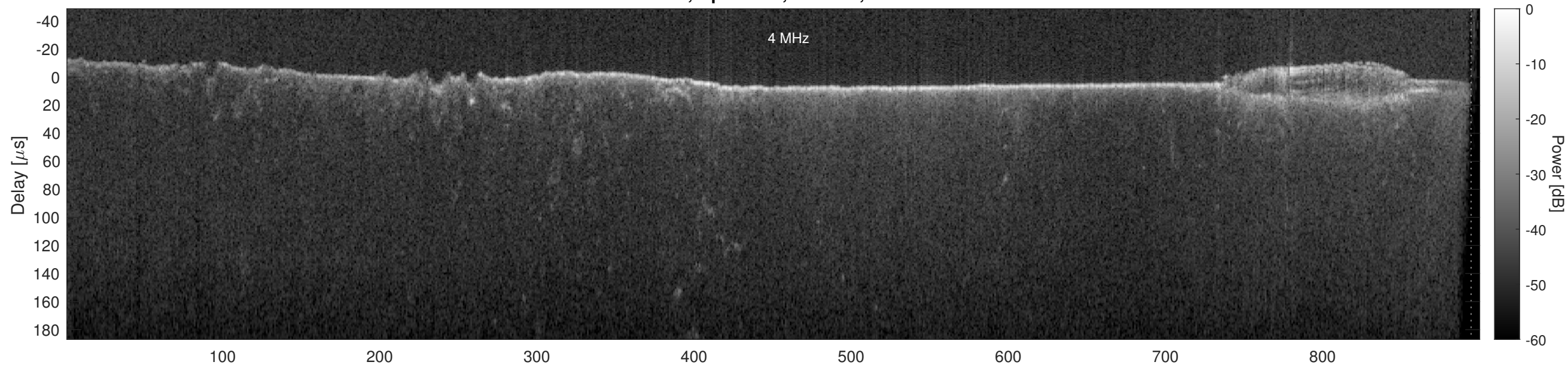
Orbit 18405, Optimized, Window, Channel 2
