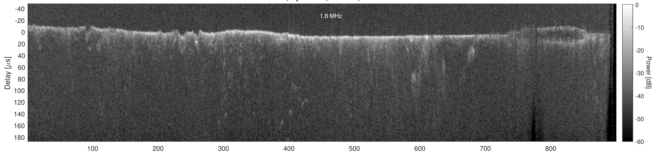
Orbit 18405, Cluttergram
