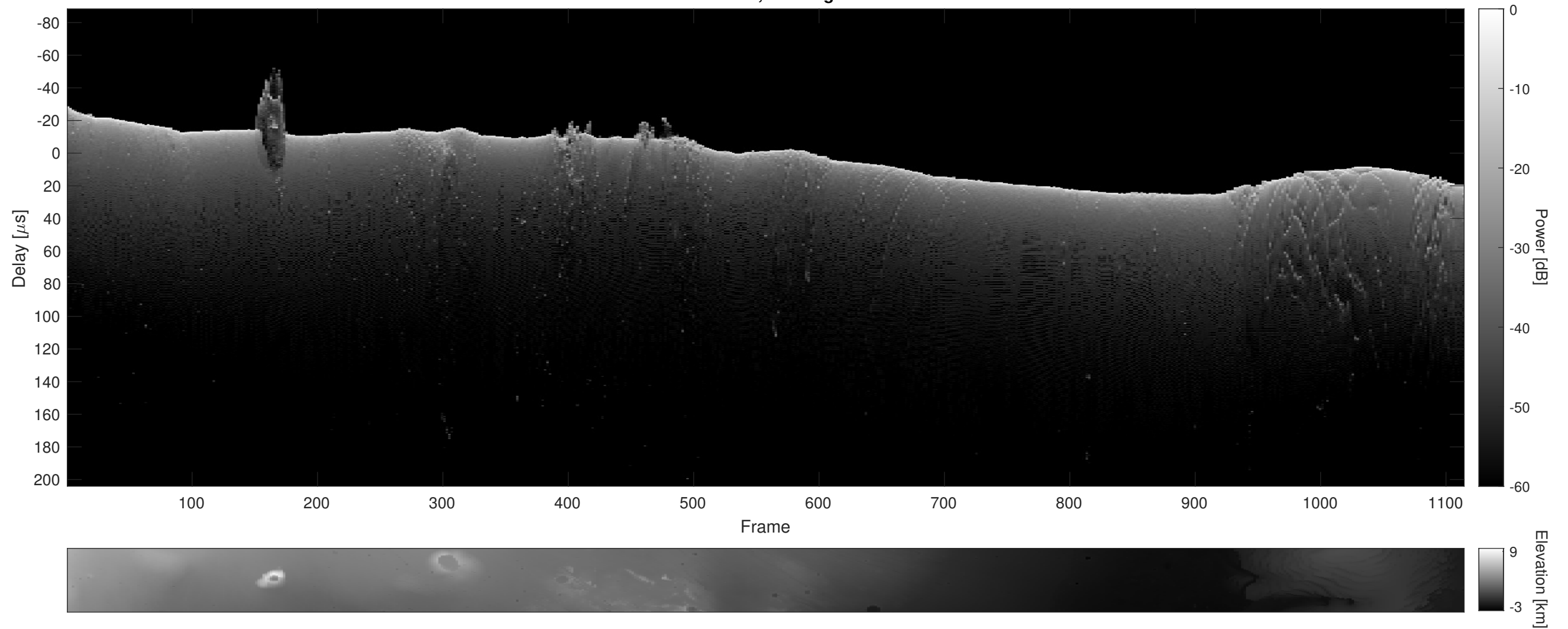
Orbit 18406, Cluttergram
