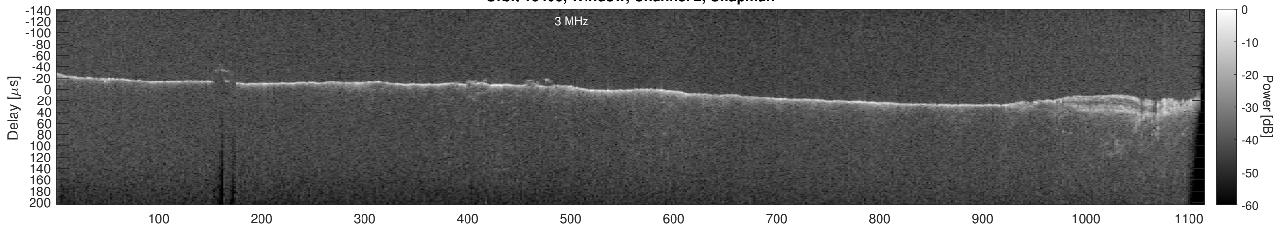
Orbit 18406, Window, Channel 2, Optimized
